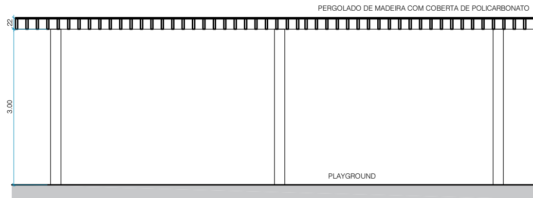
CORTE AA COBERTA PLAYGROUND ESCALA: 1/50
